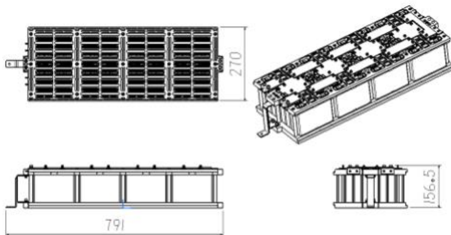
Battery Pack Structure
